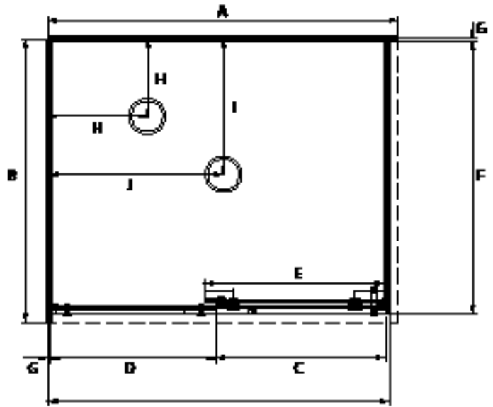
Dimension drawing depicts - Premier Frameless 2 sided LEFT HAND Fixed .
