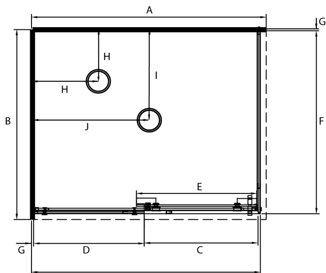
Pictured - Premier Frameless 1200 x 800 2 Sided Silva LEFT HAND Fixed SP12X8SIFWLH
